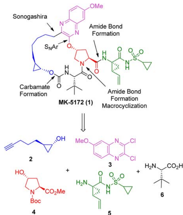
Scheme 1. Retrosynthesis of 1
