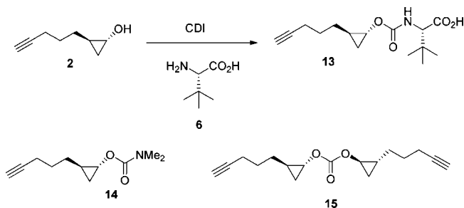
Scheme 3. L - tert -Butyl Leucine Carbamate
