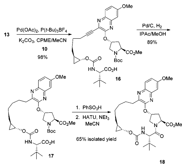
Scheme 4. Sonogashira/Macrolactamization
