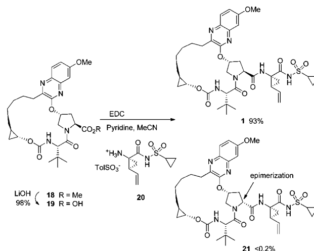
Scheme 5. End Game
