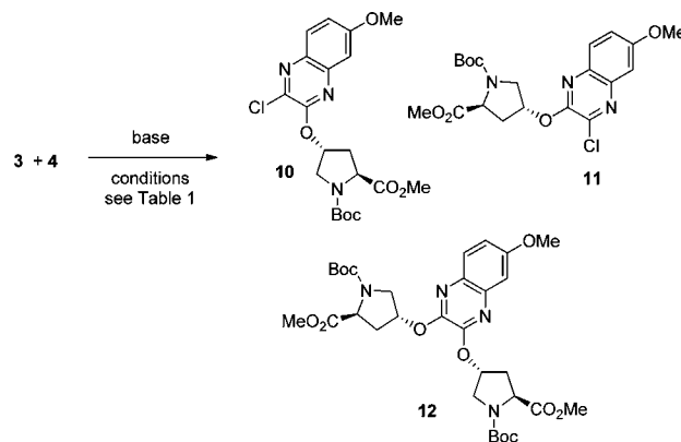
Scheme 2. Preparation of Heterocyclic Core
