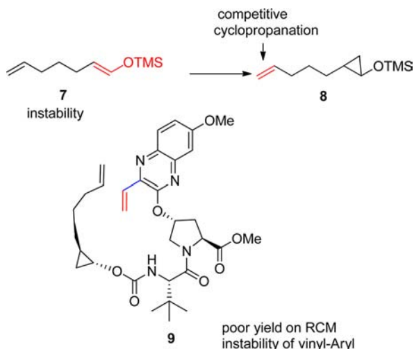
Figure 1. Major liabilities on the Med Chem Route. 5
